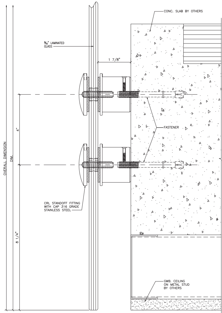
2 BOTTOM DETAIL FULL SCALE ARCH REF: N/A
