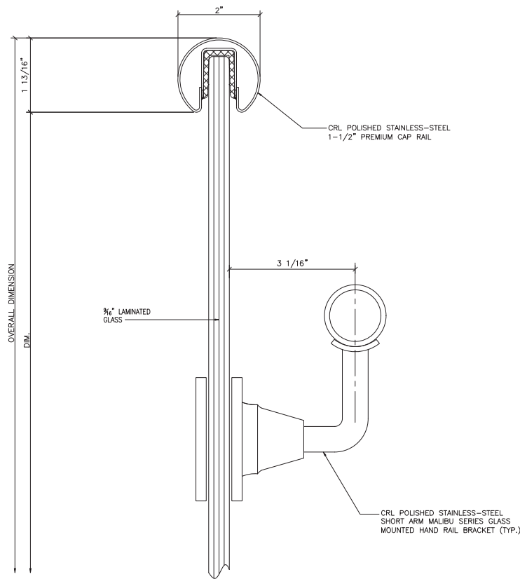
1 TOP DETAIL FULL SCALE ARCH REF: N/A
